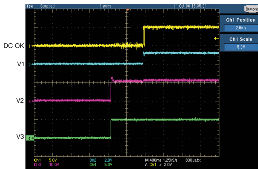
Figure 19 DC OK at AC switch on (taken from MFA350PS12)
