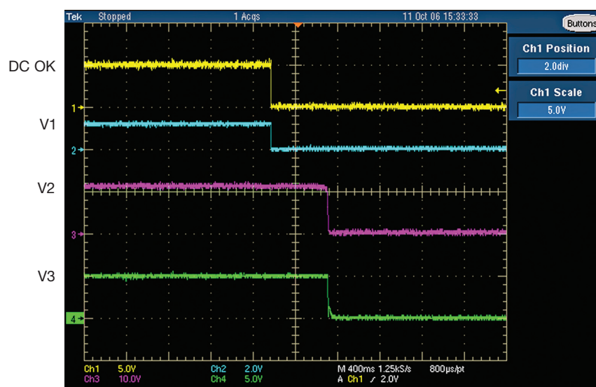
Figure 20 DC OK at AC switch off (taken from MFA350PS12)
