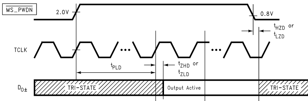
Figure 6. Serializer PLL lock Time and \overline{\text{MS\_PWDN}} TRI-STATE Delays
