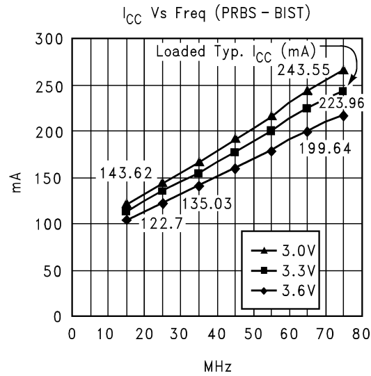
Figure 10. I_{CC} vs Freq
