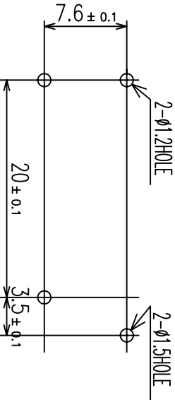
DRILLING DIAGRAM(2/1) (BOTTOM VIEW)
