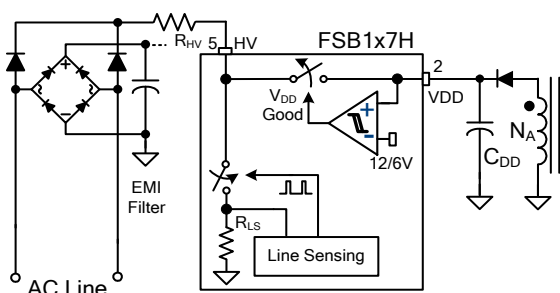
Figure 18. Startup Circuit
