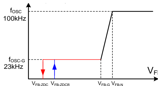
Figure 25. PWM Frequency
