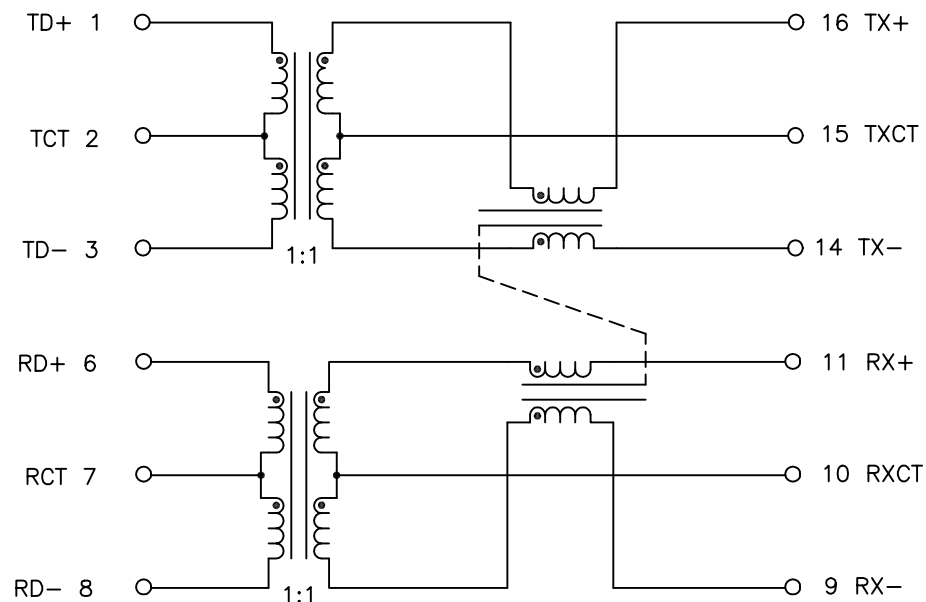
SCHEMATIC
