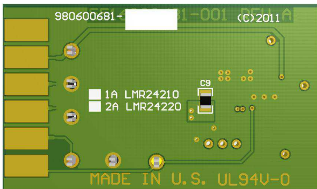
Bottom View
