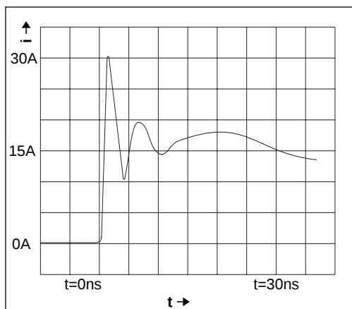
Figure 12. ESD Test Waveform for EN61000-4-2
