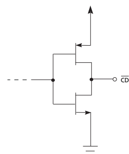
Figure 3-5: \overline{CD} Circuit
