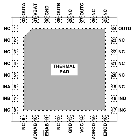
ISL1540 [32 Ld QFN (8mm x 8mm)] TOP VIEW
