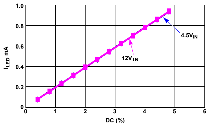
FIGURE 9. CURRENT LINEARITY vs LOW LEVEL PWM DIMMING DUTY CYCLE vs V_{IN}
