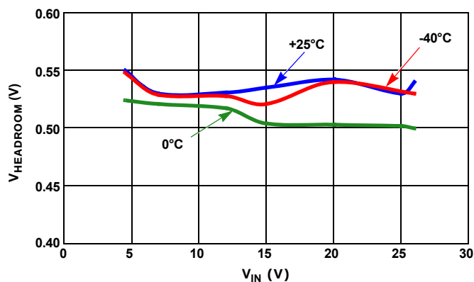
FIGURE 11. V_{HEADROOM} vs V_{IN} vs TEMPERATURE AT 20mA
