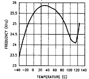
Short Circuit Frequency vs Temperature
