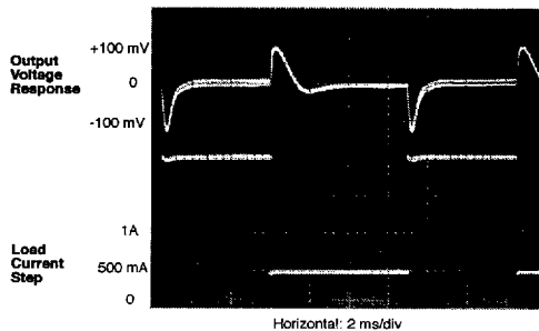
FIGURE 35. V_{OUT} Response to Load Current Step
