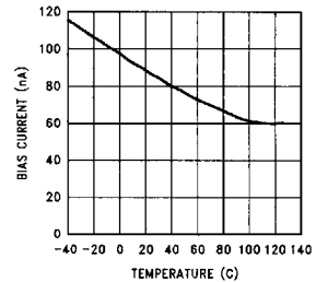
Feedback Pin Bias Current vs Temperature
