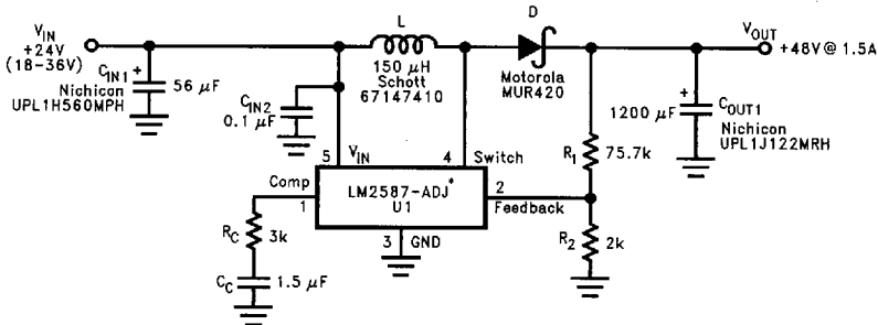
FIGURE 40. +24V to +48V Boost Regulator
