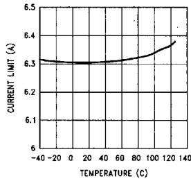
Current Limit vs Temperature
