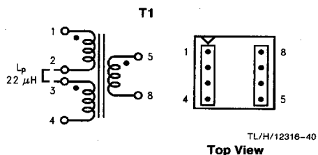
FIGURE 25. Renco RL-5530
