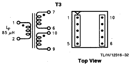
FIGURE 17. Coilcraft Q4343-B
