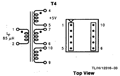
FIGURE 18. Coilcraft Q4344-B
