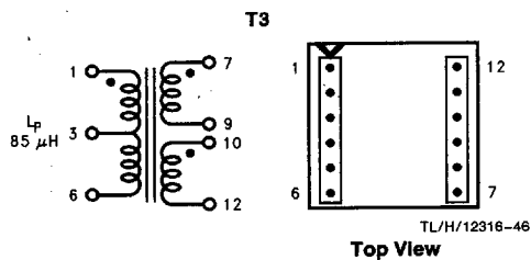
FIGURE 27. Renco RL-5534
