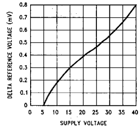
ΔReference Voltage vs Supply Voltage
