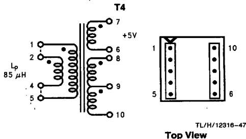
FIGURE 32. Schott 67140930
