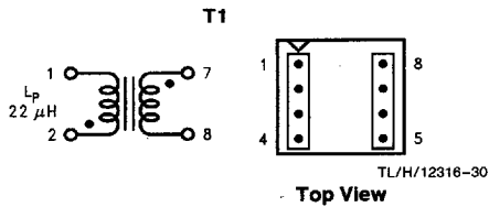
FIGURE 15. Coilcraft Q4434-B
