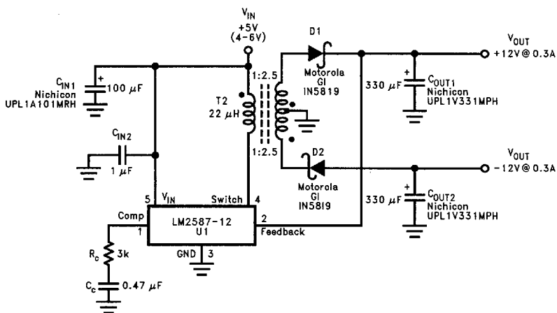
FIGURE 10. Dual-Output Flyback Regulator
