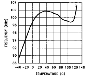
Oscillator Frequency vs Temperature
