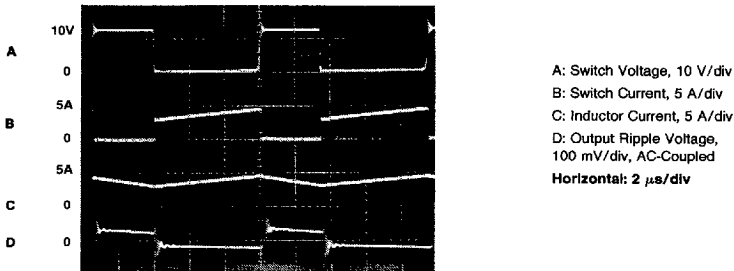
FIGURE 34. Switching Waveforms
