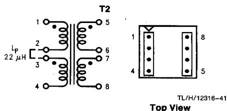
FIGURE 26. Renco RL-5531
