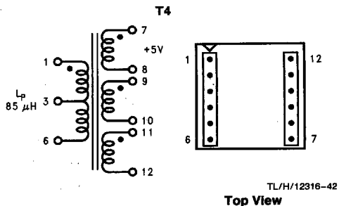
FIGURE 28. Renco RL-5535
