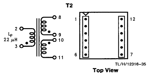
FIGURE 20. Coilcraft Q4436-B (Surface Mount)
