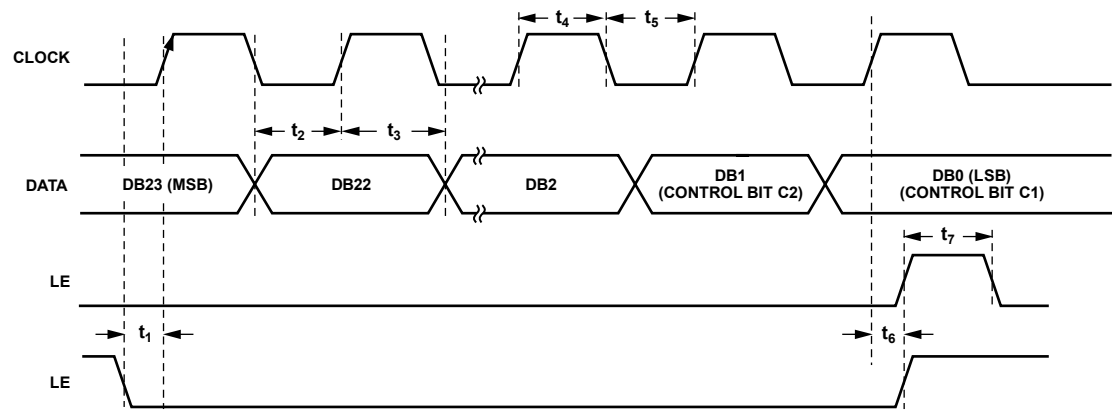
Figure 2. Timing Diagram
