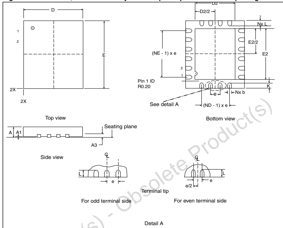
Figure 105. QFN 5x6, 20-terminal very thin fine pitch quad flat no-lead package
