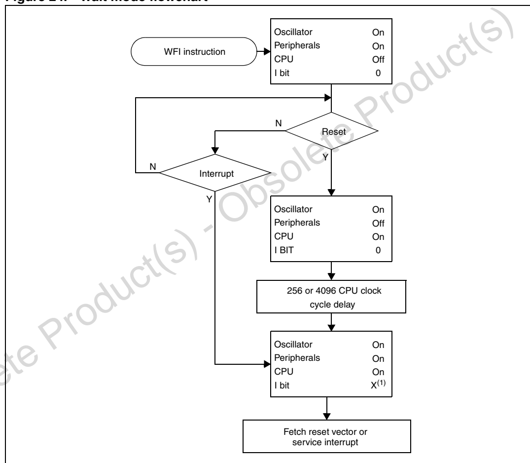
Figure 24. Wait mode flowchart
