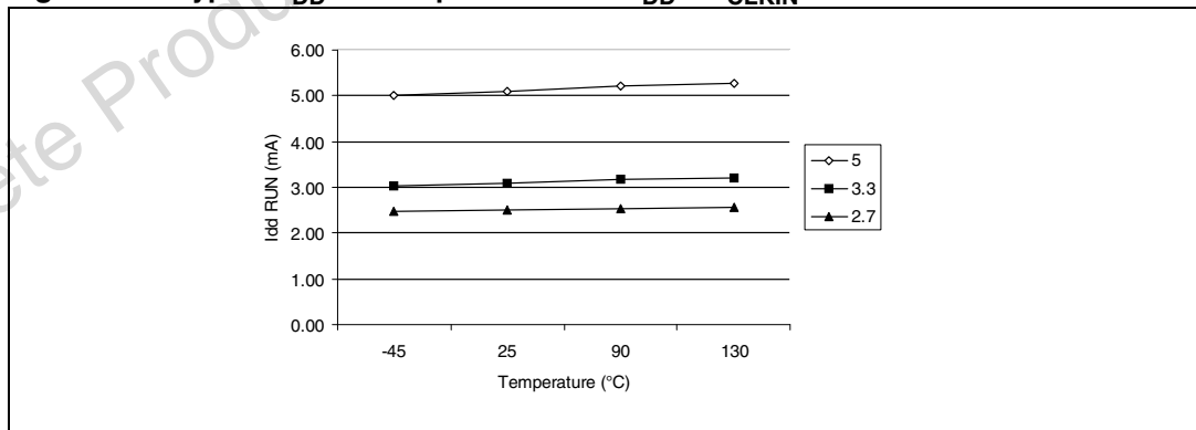
Figure 83. Typical I_{DD} vs. temperature and V_{DD} at f_{CLKIN} = 16\text{ MHz}
