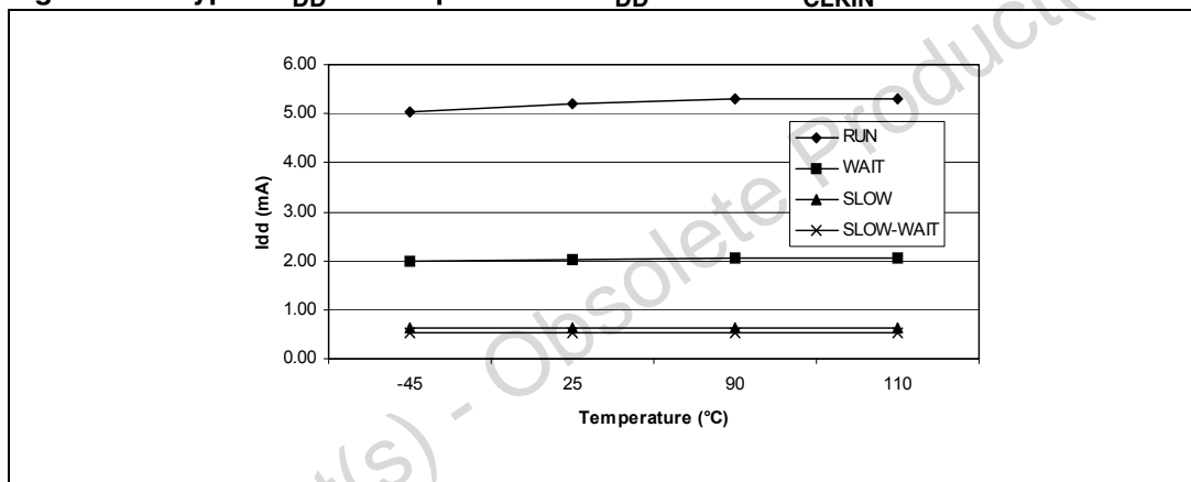
Figure 83. Typical I_{DD} vs. temperature and V_{DD} at f_{CLKIN} = 16\text{ MHz}
