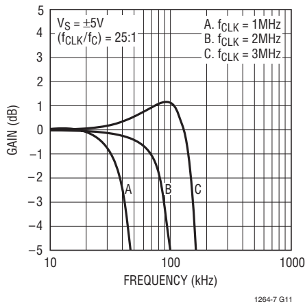
Passband Gain vs f_{CLK} at 85^\circ C
