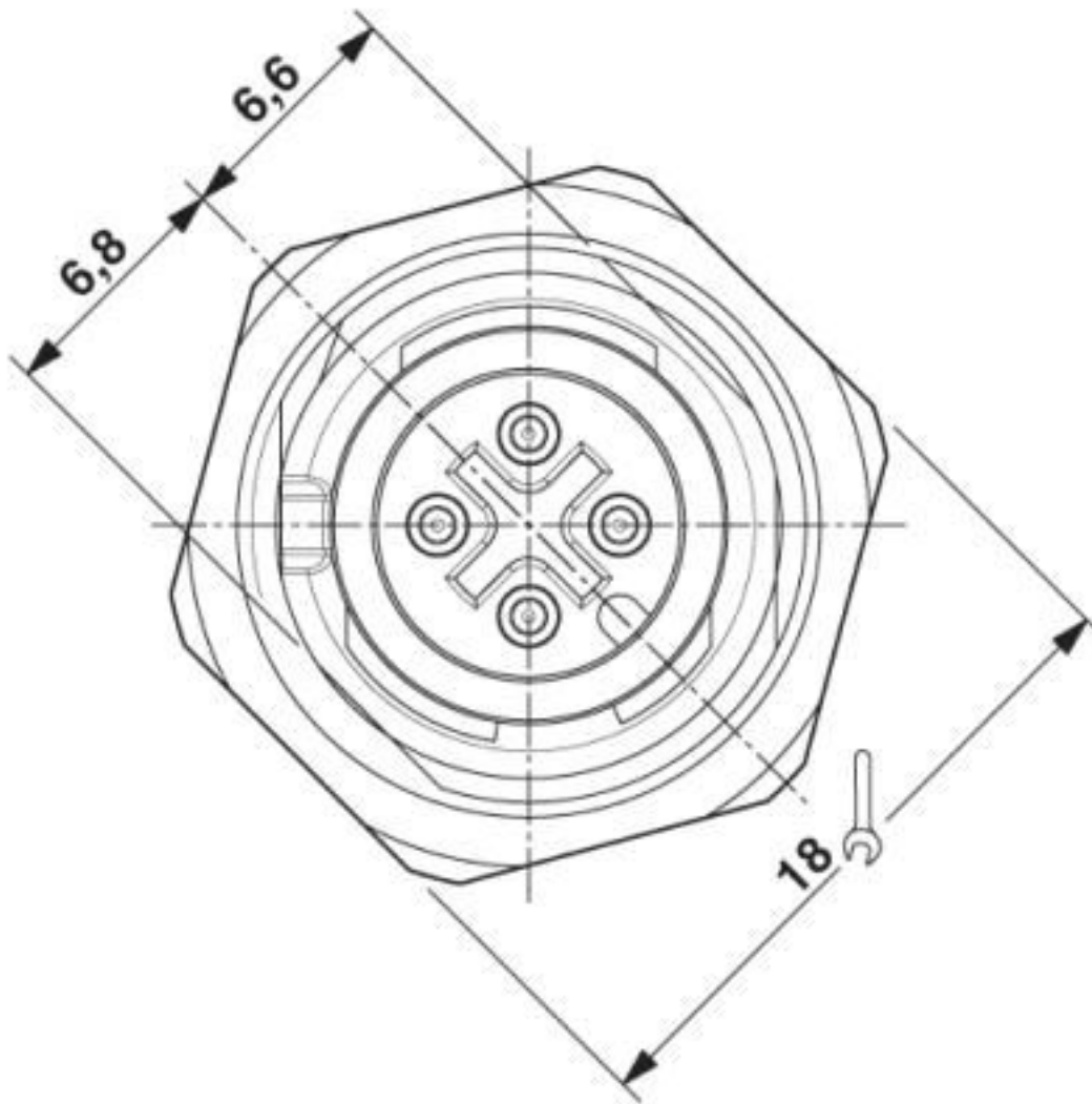
Dimensional drawing
