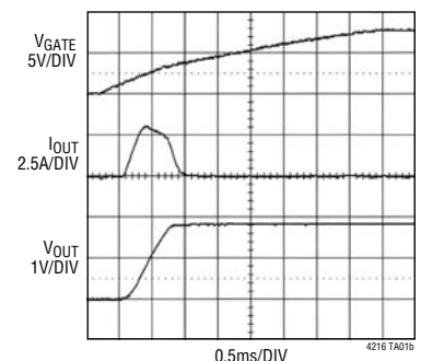
Normal Power-Up with Soft-Start
