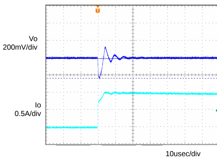
Fig.4 Transient Response (1.0→0A) Co=1\mu F , T_a=25^\circ C
