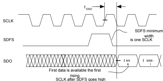
Figure xx. Timing for Serial Output Port (SBM=1)
