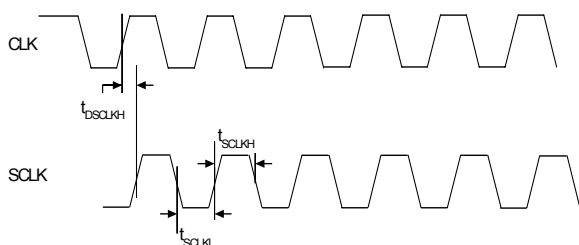
Figure xx. SCLK Switching Characteristics (Divide by 1)
