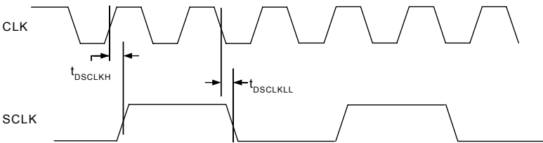
Figure x. SCLK Switching Characteristics (Divide by 3 or ODD integer)
