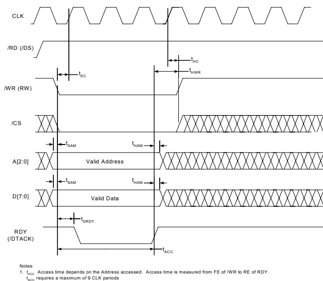
Figure 16. INM Microport Write Timing Requirements.
