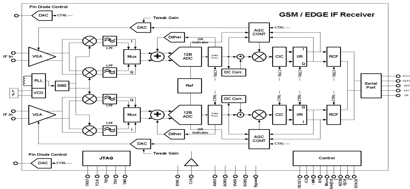
Figure 1. AD6650 Functional Block Diagram
