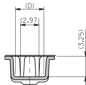
SECT:X-X (SCALE:4-1)
