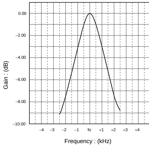
Fig.6 BPF characteristic
