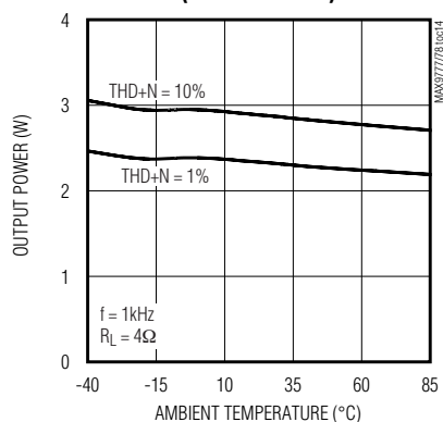
OUTPUT POWER vs. AMBIENT TEMPERATURE (SPEAKER MODE)
