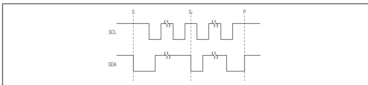
Figure 4. START/STOP Conditions
