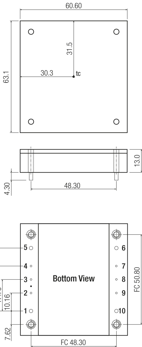
Dimension Drawing (mm)
