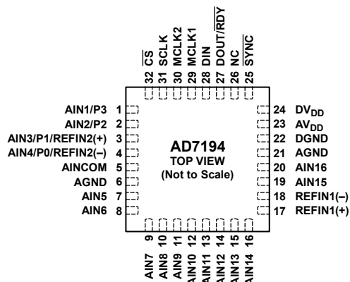
Figure 5. Pin Configuration
