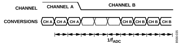
Figure 36. Sinc 3 Channel Change
