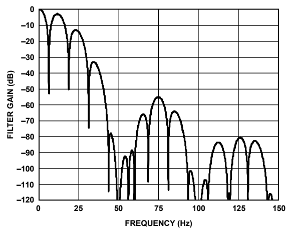
Figure 47. Sinc 4 Filter Response (FS[9:0] = 96, Chop Enabled, REJ60 = 1)
