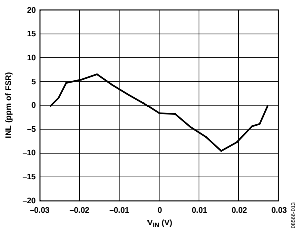
Figure 13. INL (Gain = 128)
