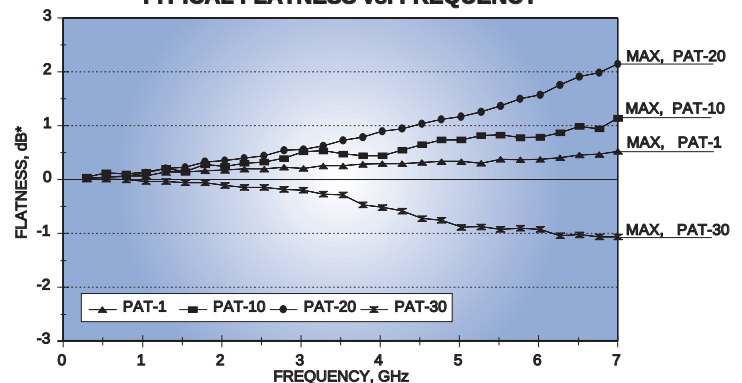
TYPICAL FLATNESS vs. FREQUENCY
