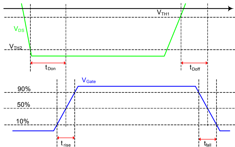
Fig. 15 - Timing Diagrams
