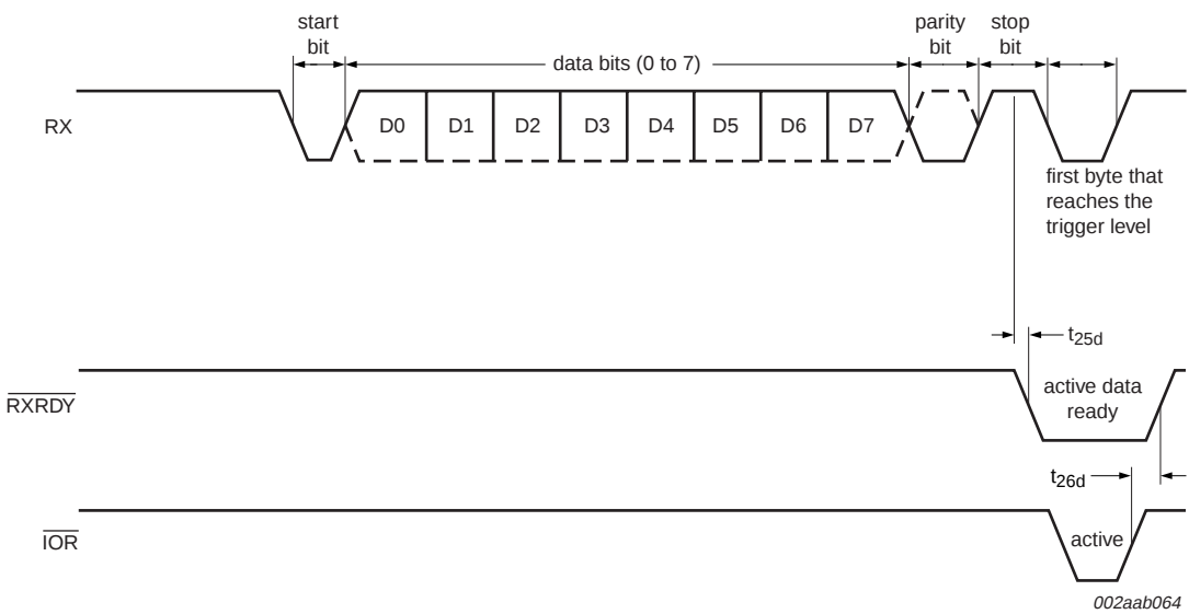
Fig 16. Receive ready timing in FIFO mode
