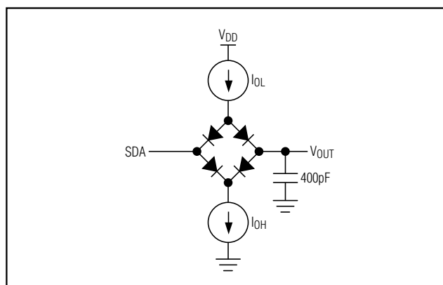
Figure 2. Load Circuits
