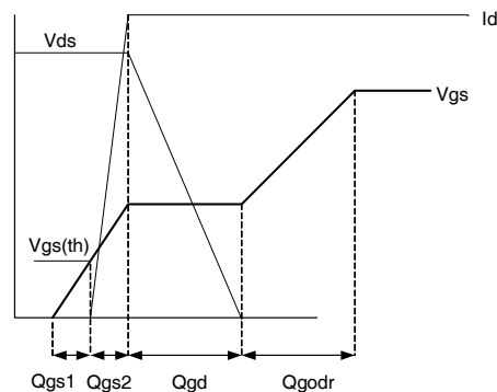
Fig 31b. Gate Charge Waveform
