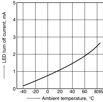
6.-(2) LED turn off current vs. ambient temperature characteristics Sample: AQV253H, AQV254H, AQV256H; Load voltage: Max. (DC); Continuous load current: Max. (DC)
