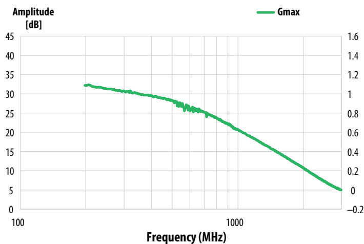
Figure 12: Gain Chart
