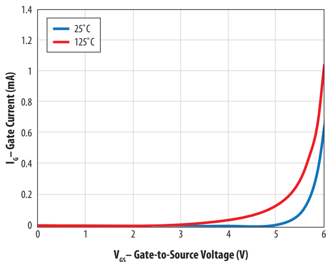
Figure 10: Gate Current
