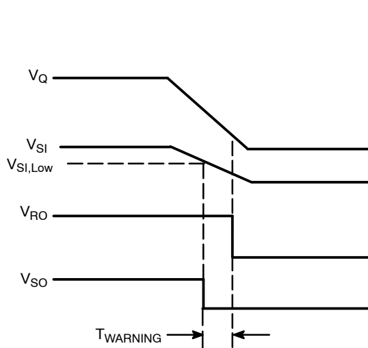
Figure 42. SO Warning Timing Waveform
