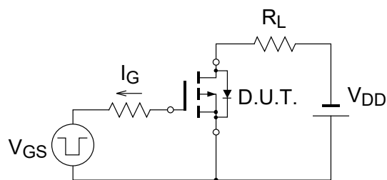
Test Circuit
