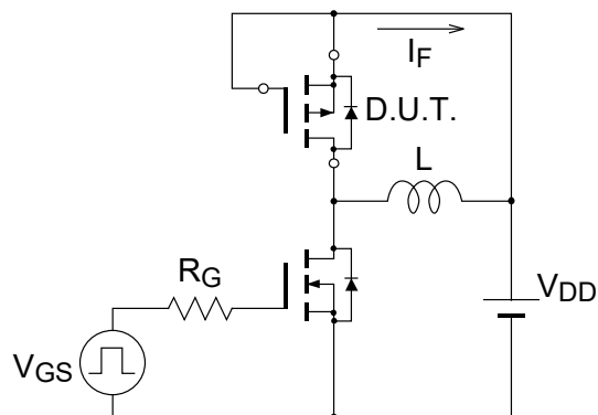
Test Circuit
