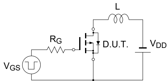
Test Circuit
