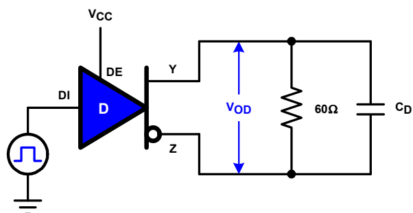
Figure 7. Measurement of Driver Data Rate
