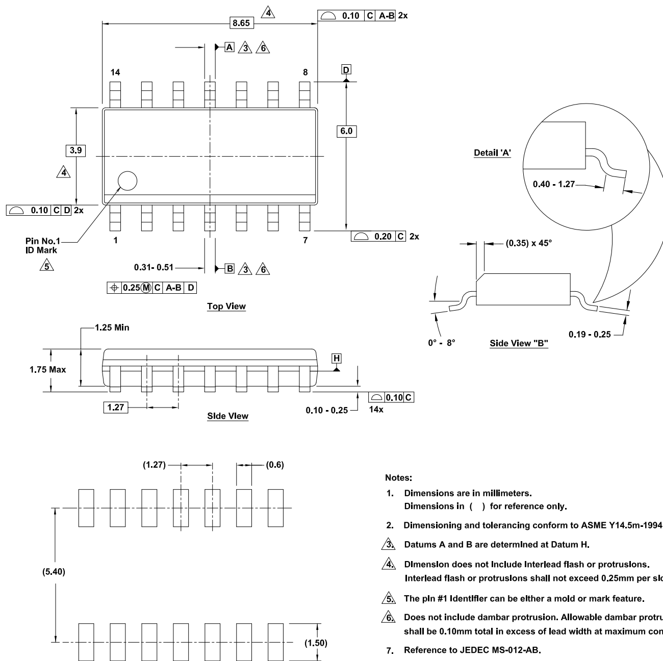
Typical Recommended Land Pattern
