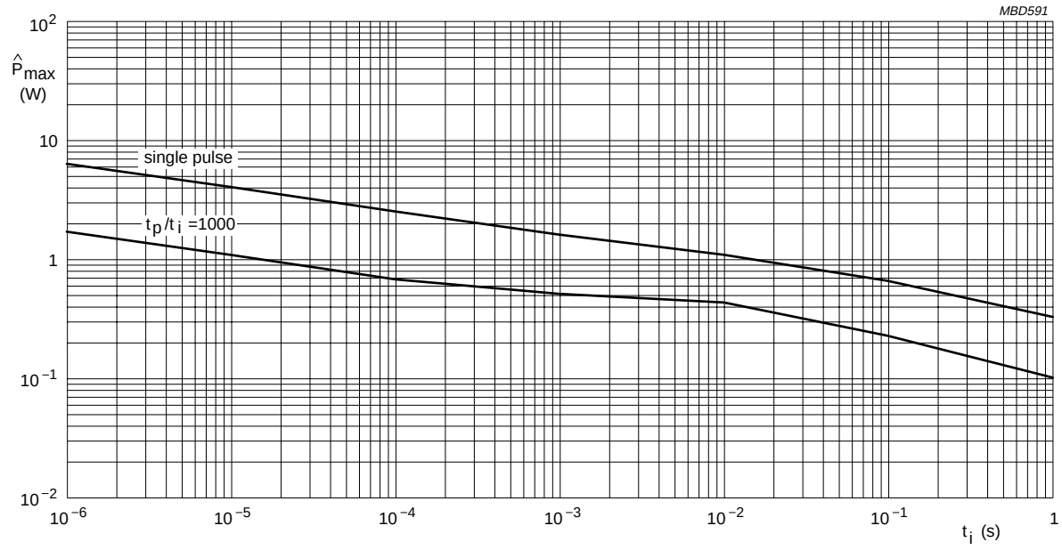
Fig.10 Pulse on a regular basis for type: RC21 ; maximum permissible peak pulse power ( \hat{P}_{max} ) as a function of pulse duration for R \leq 10\text{ k}\Omega , single pulse and repetitive pulse t_p/t_i = 1000 .
