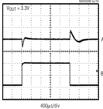
LOAD-TRANSIENT RESPONSE (MAX5090AATE)
