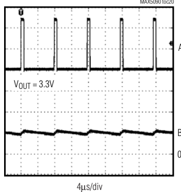
LX WAVEFORMS (MAX5090AATE)
