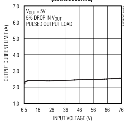
OUTPUT CURRENT LIMIT vs. INPUT VOLTAGE (MAX5090BATE)
