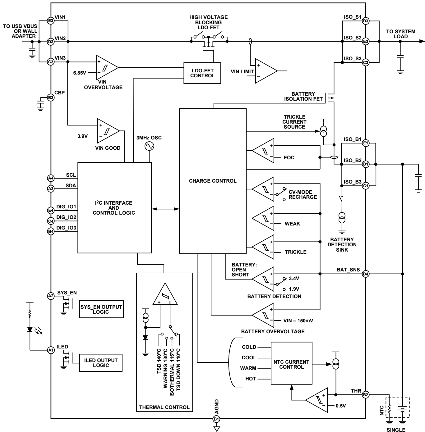
Figure 29. Block Diagram
