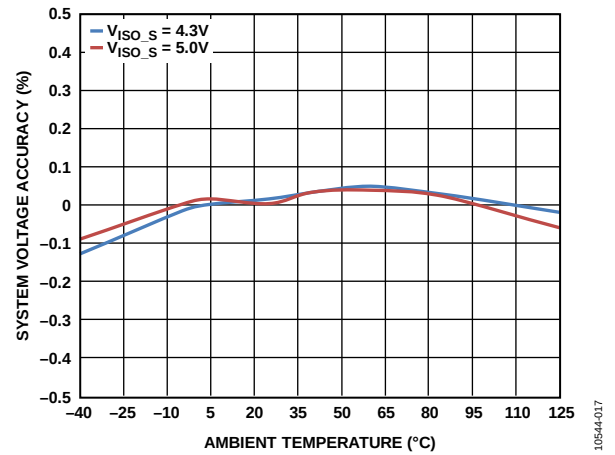
Figure 17. System Voltage vs. Temperature, Trickle Charge Mode, V_{ISO\_S} = 4.3 V and V_{INx} = 5.0 V, or V_{ISO\_S} = 5.0 V and V_{INx} = 6.0 V
