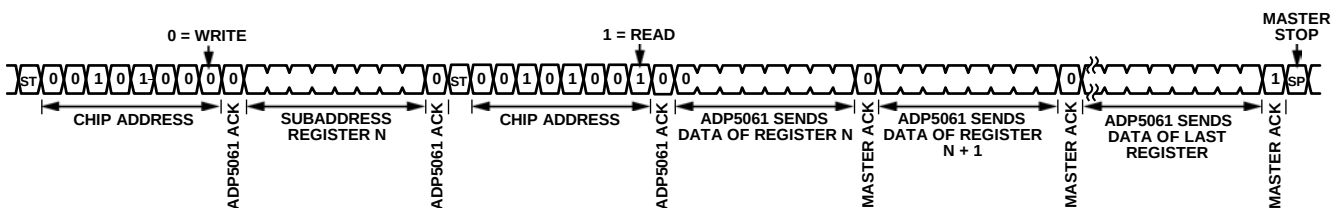
Figure 37. I 2 C Multiple Register Read Sequence
