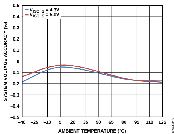
Figure 16. LDO Mode Voltage vs. Ambient Temperature, Load = 100 mA, V_{IN} = 5.5 V
