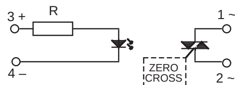
Figure 2 — FS relays
