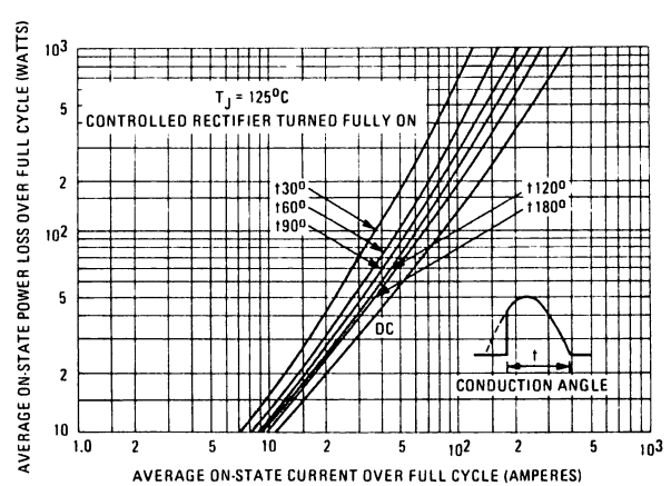
Fig. 4 – Maximum High-Level On-State Power Loss Vs. Current (Sinusoidal Current Waveform)
