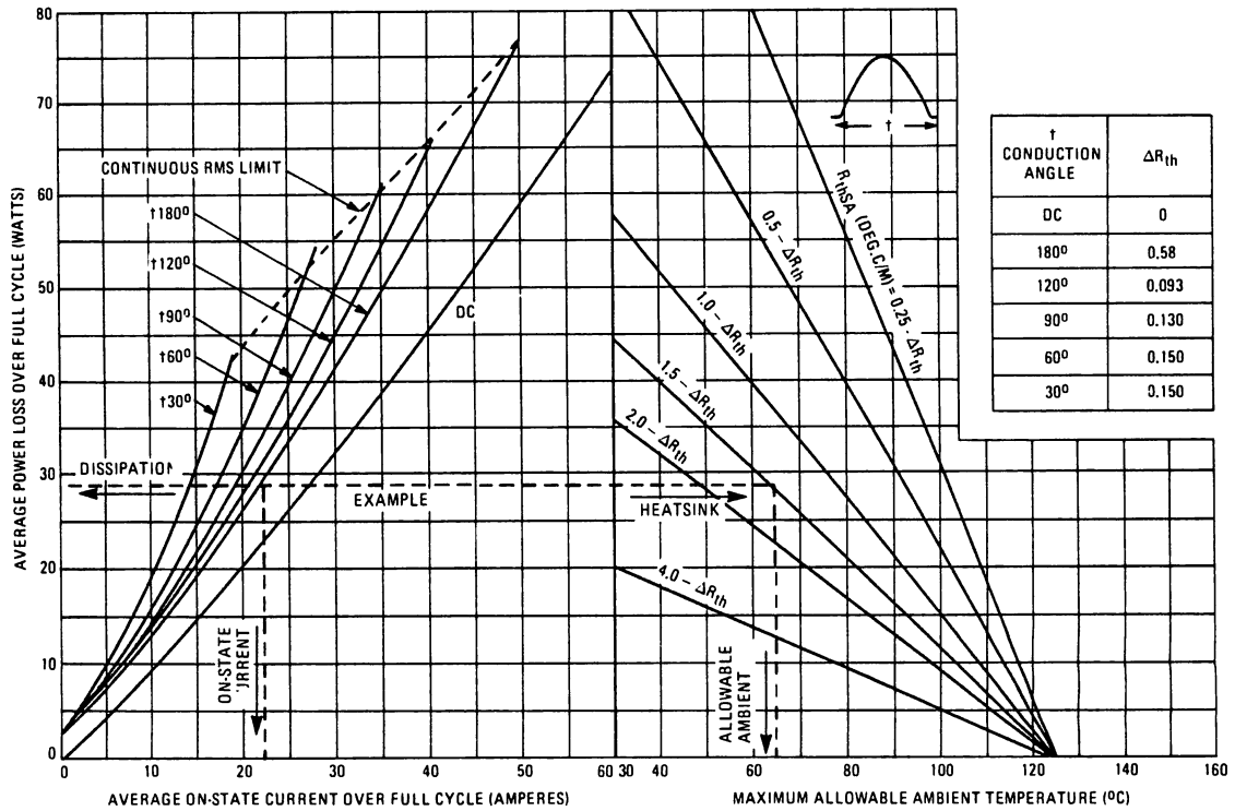
Fig. 11 – Thermal Nomogram (Sinusoidal Current Waveform, 40 to 400 Hz)
