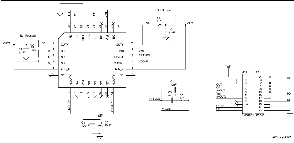
Figure 1. Internal schematic
