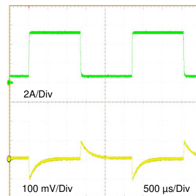
Figure 5-40. Output Ripple
