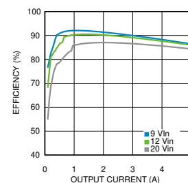
Efficiency 5V Output at 25^{\circ}\text{C} Ambient
