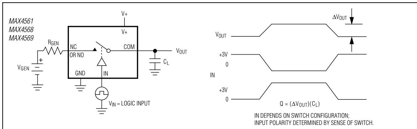
Figure 3. Charge Injection
