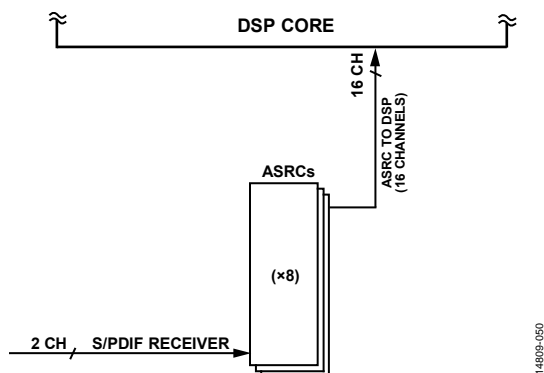
Figure 58. Example ASRC Routing for Asynchronous Input to the DSP Core
