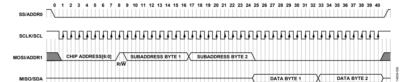
Figure 37. SPI Slave Read Clocking (Single Word Mode, Two Bytes)
