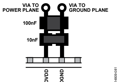
Figure 85. Layout for Multiple Power Supply Bypass Capacitors
