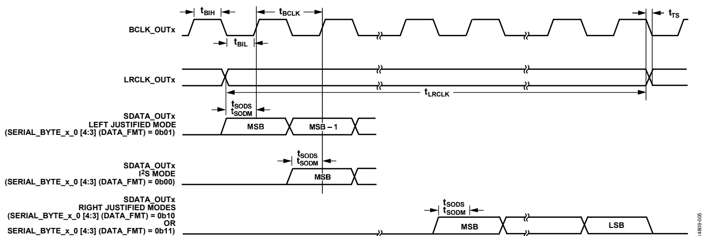
Figure 5. Serial Output Port Timing Specifications
