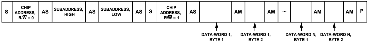
Figure 33. Simplified Burst Mode I 2 C Read Sequence
