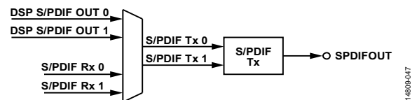
Figure 72. S/PDIF Transmitter Source Selection
