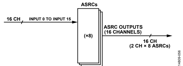
Figure 64. Example ASRC Routing, Bypassing DSP Core
