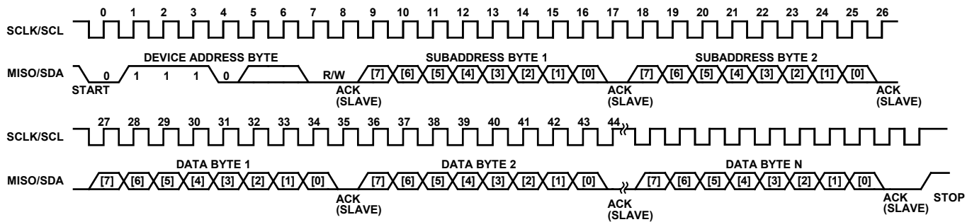
Figure 28. I²C Slave Burst Mode Write Operation (N Bytes)
