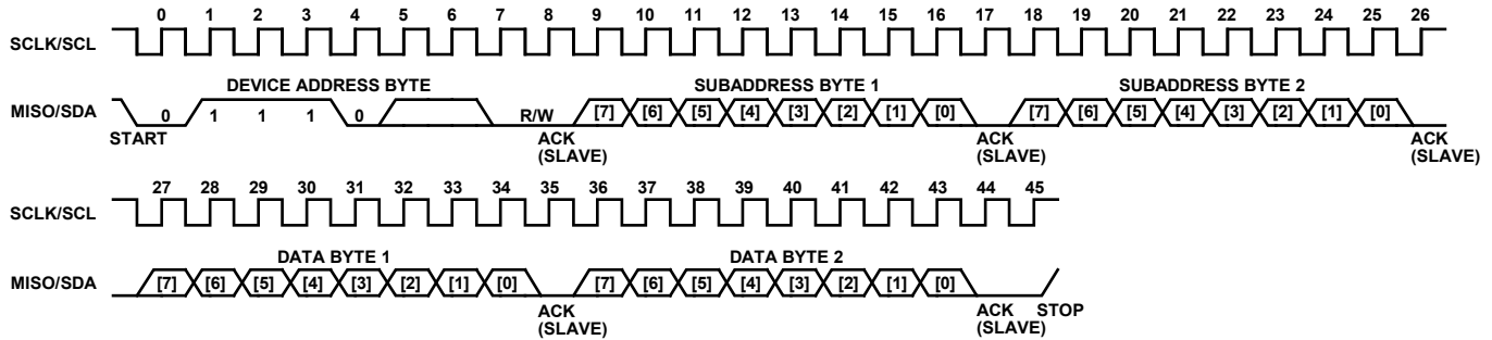
Figure 27. I²C Slave Single Word Write Operation (Two Bytes)
