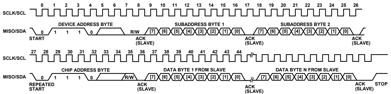
Figure 29. I²C Slave Burst Mode Read Operation (N Bytes)
