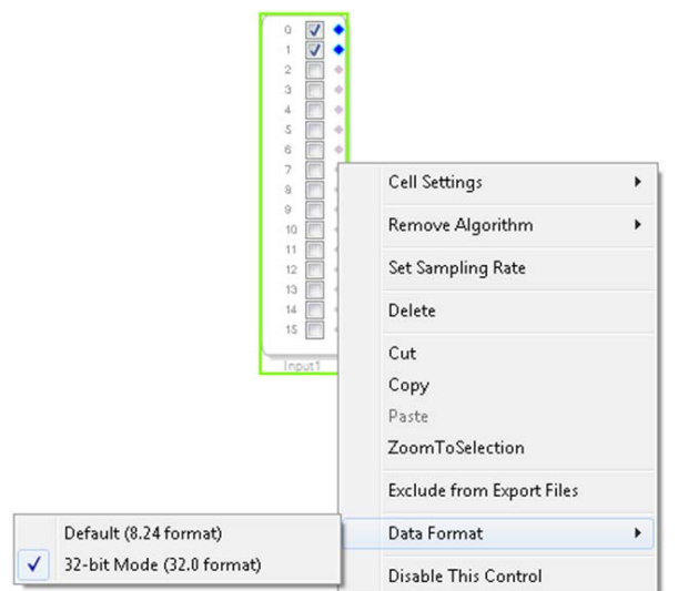
Figure 43. Selecting 32-Bit Serial Input Mode in SigmaStudio
