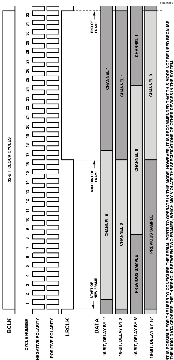
Figure 56. Serial Audio Data Formats; Two Channels, 16 Bits per Channel
