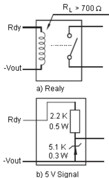
Figure 1 Rdy connection
