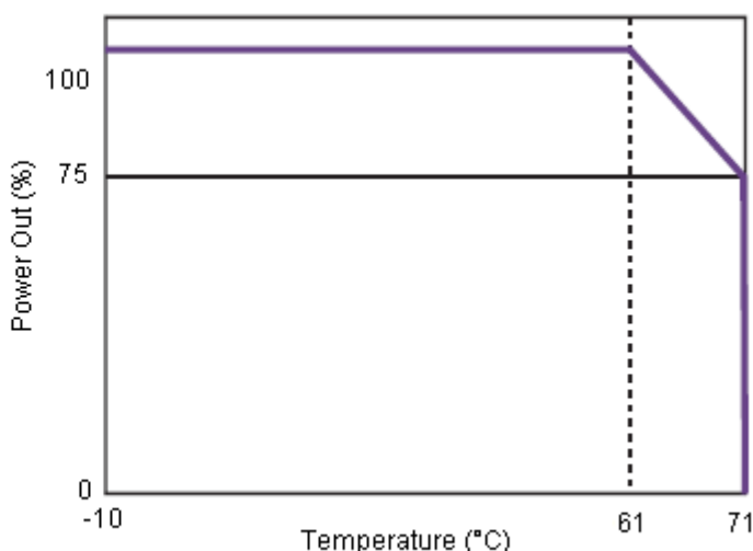
Derating
