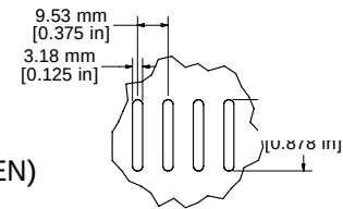
DETAIL KK
