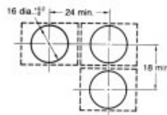
Panel cutout (top view)
