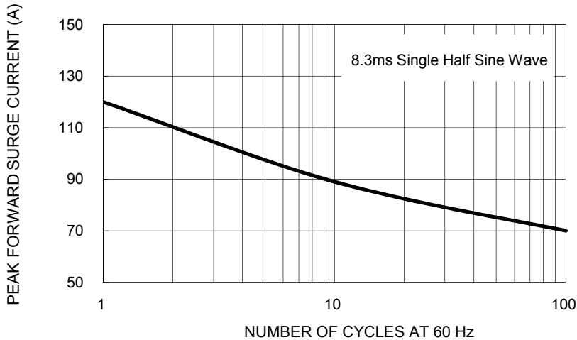
FIG. 2 MAXIMUM NON-REPETITIVE FORWARD SURGE CURRENT
