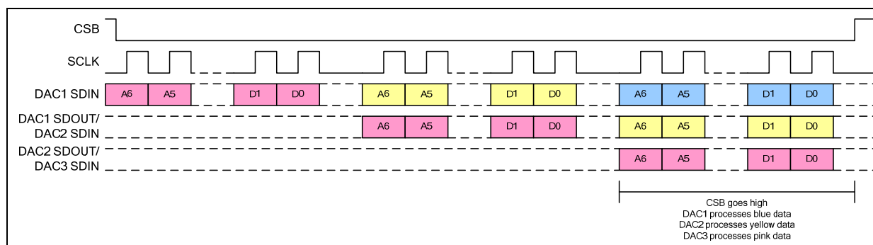
Figure 12 Daisy Chain Control Interface Example for Three WM8741 Devices
