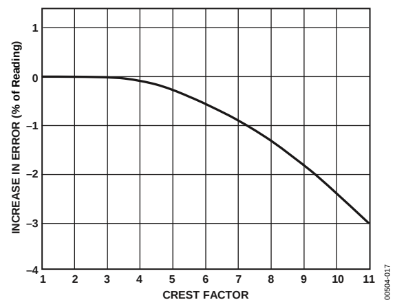
Figure 9. Error vs. Crest Factor
