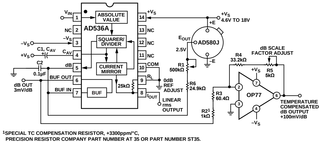
Figure 7. dB Connection
