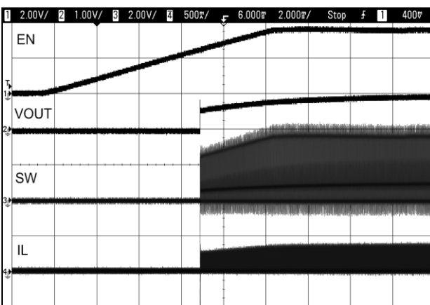
Figure 30. Cold-Start Transient Response from 0 mA to 100 mA
