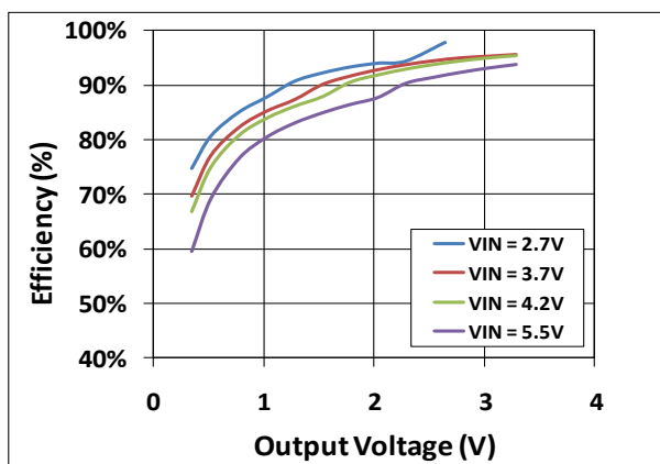
Figure 11. Efficiency vs. Output Voltage vs. Input Voltage, f_{SW} = 3\text{ MHz} , R_{PA} = 7\text{ }\Omega
