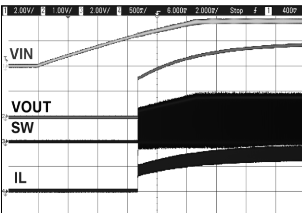
Figure 32. Cold-Start Transient Response from 0 mA to 800 mA
