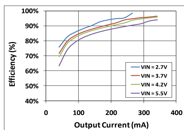
Figure 10. Efficiency vs. Output Current vs. Input Voltage, f_{SW} = 3\text{ MHz} , R_{PA} = 10\text{ }\Omega
