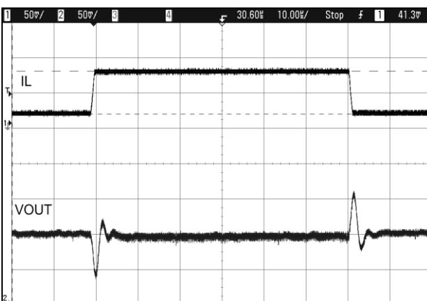
Figure 22. Load Transient, 200\text{ mA} to 800\text{ mA} , V_{OUT} = 2.5\text{ V}
