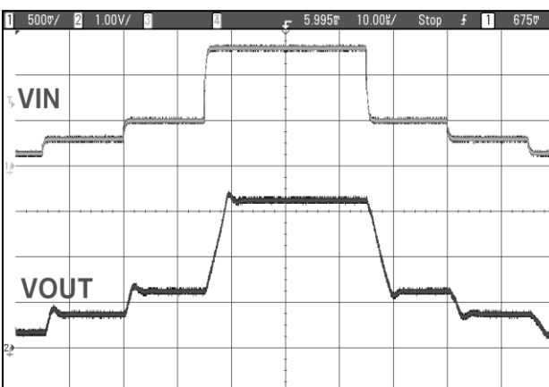
Figure 16. Rise Times for 300 mV, 500 mV, and 2 V \Delta V_{OUT} ( V_{IN} = 3.7\text{ V} )
