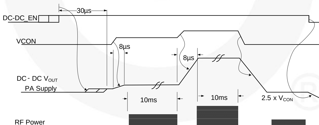
Figure 40. Timing Diagram for 3G/4G Transmitters
