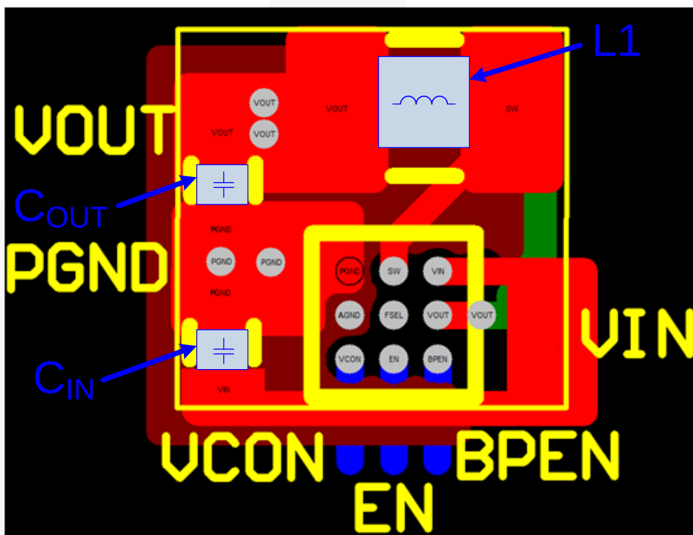
Figure 41. Recommended PCB Layout
