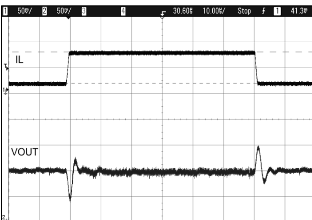
Figure 20. Load Transient, 200\text{ mA} to 800\text{ mA} , V_{OUT} = 1.0\text{ V}
