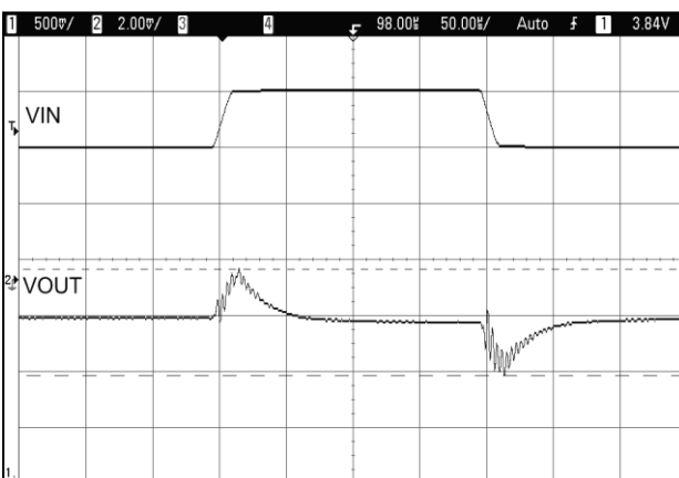
Figure 18. Line Transient V_{IN} = 3.7\text{ V} to 4.2\text{ V} , V_{OUT} = 1.0\text{ V} , 10\text{ }\Omega Load, 50\text{ }\mu\text{s/div} .
