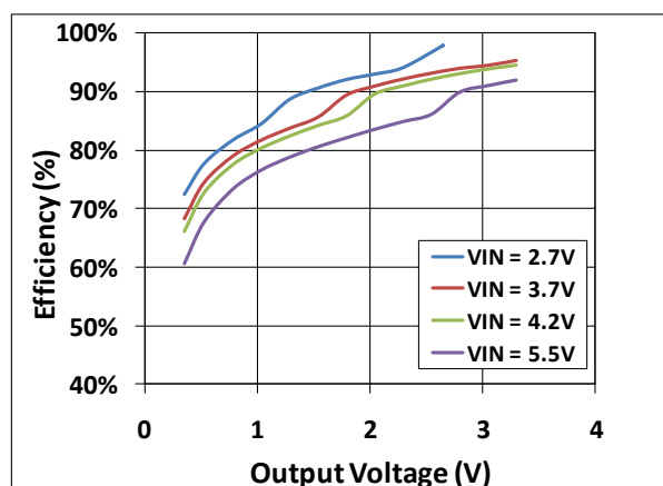
Figure 7. Efficiency vs. Output Voltage vs. Input Voltage, f_{SW} = 6\text{ MHz} , R_{PA} = 7\text{ }\Omega
