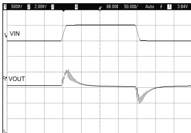
Figure 17. Line Transient V_{IN} = 3.7\text{ V} to 4.2\text{ V} , V_{OUT} = 2.5\text{ V} , 10\text{ }\Omega Load, 50\text{ }\mu\text{s/div} .
