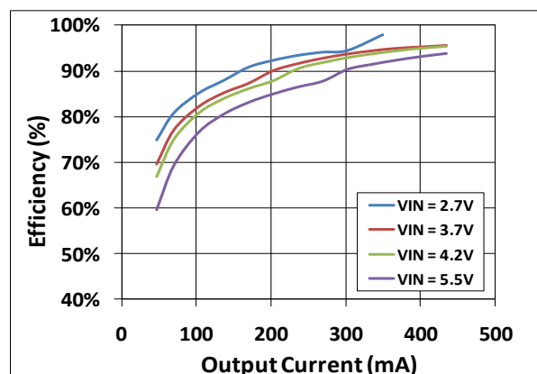
Figure 9. Efficiency vs. Output Current vs. Input Voltage, f_{SW} = 3\text{ MHz} , R_{PA} = 7\text{ }\Omega
