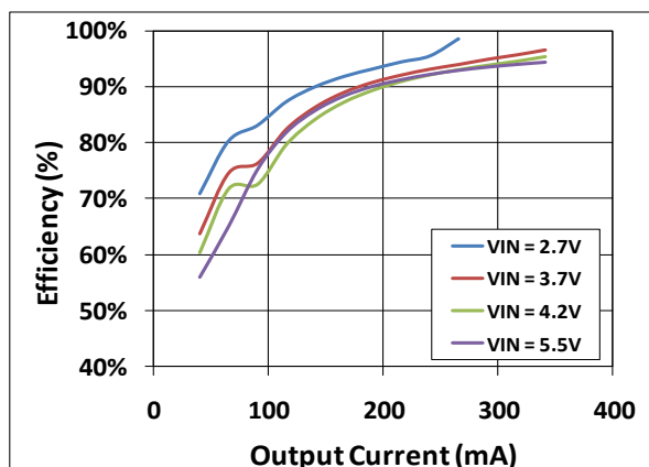
Figure 6. Efficiency vs. Output Current vs. Input Voltage, f_{SW} = 6\text{ MHz} , R_{PA} = 10\text{ }\Omega
