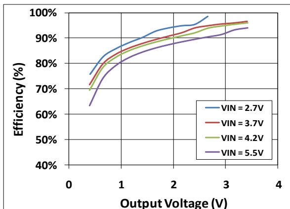
Figure 12. Efficiency vs. Output Voltage vs. Input Voltage, f_{SW} = 3\text{ MHz} , R_{PA} = 10\text{ }\Omega
