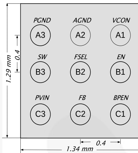
Figure 4. Top-Through View, Bumps Face Up
