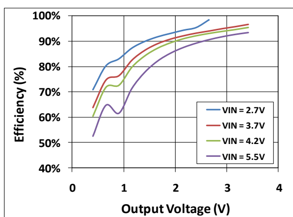
Figure 8. Efficiency vs. Output Voltage vs. Input Voltage, f_{SW} = 6\text{ MHz} , R_{PA} = 10\text{ }\Omega
