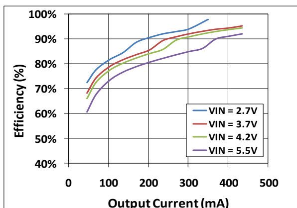
Figure 5. Efficiency vs. Output Current vs. Input Voltage, f_{SW} = 6\text{ MHz} , R_{PA} = 7\text{ }\Omega
