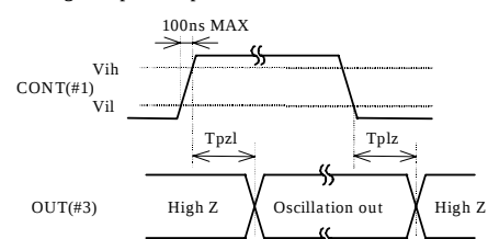
Fig.4 Input output condition
